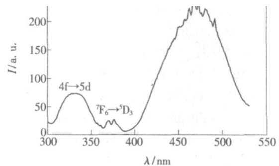
图 4 以 537 nm 为监测波长, TAG:Ce 荧光粉的激发光谱 Fig 4 Excitation spectra of TAG:Ce powder monitored at 537 nm.
